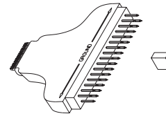
Figure 3.5. Wedge adapters connect to multiple pins of 0.5 mm or 0.65 mm QFP ICs. Refer to "Probing Solutions for Agilent Technologies Logic Analysis Systems," publication number 5968-4632E, for specific part numbers.
