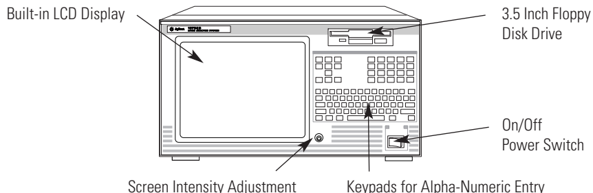
Figure 6.4. Agilent 16702A front panel.
