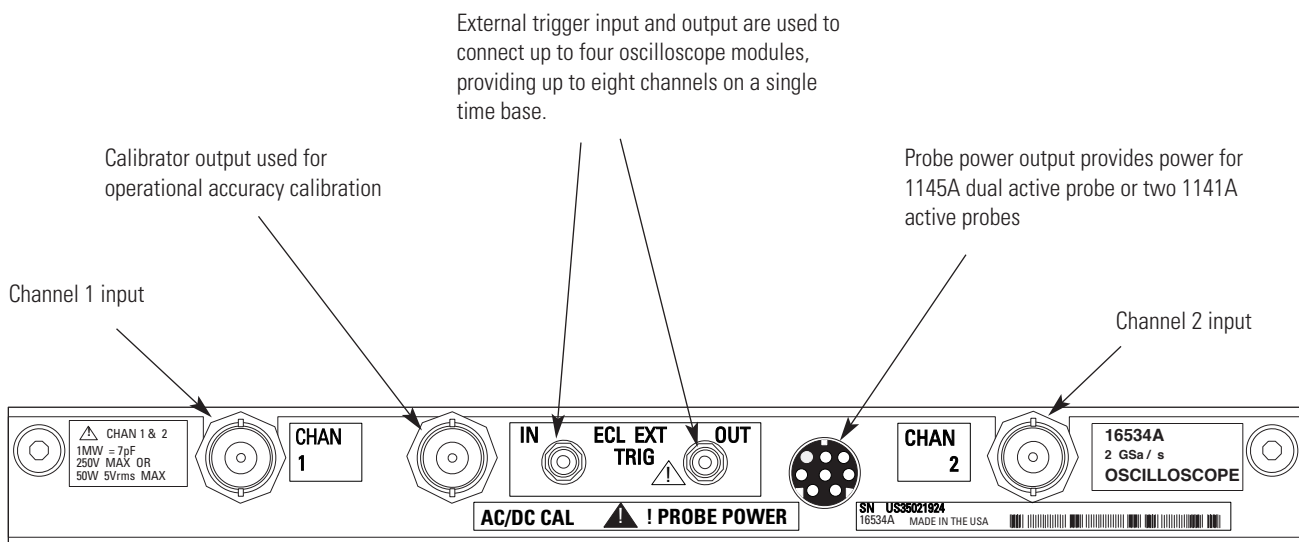
Figure 4.7. Connector panel of the 16533A and 16534A oscilloscope modules.
