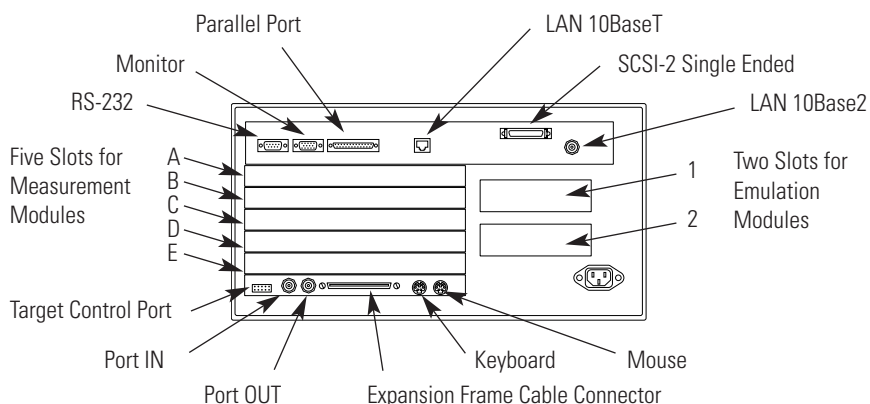
Figure 6.5. Back panel for Agilent models 16700A and 16702A.
