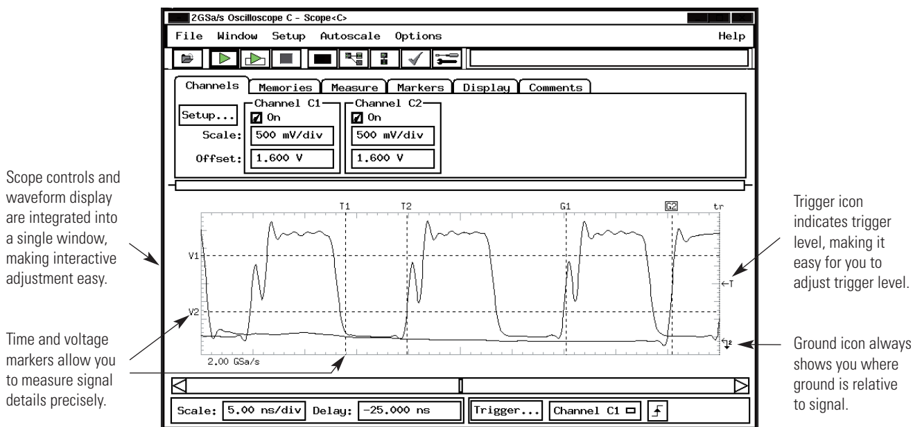
Figure 4.5. All primary oscilloscope control settings, including scale factors and trigger settings, are visible simultaneously.
