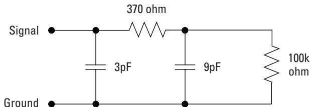
Figure 6.10. E5346A equivalent load.
