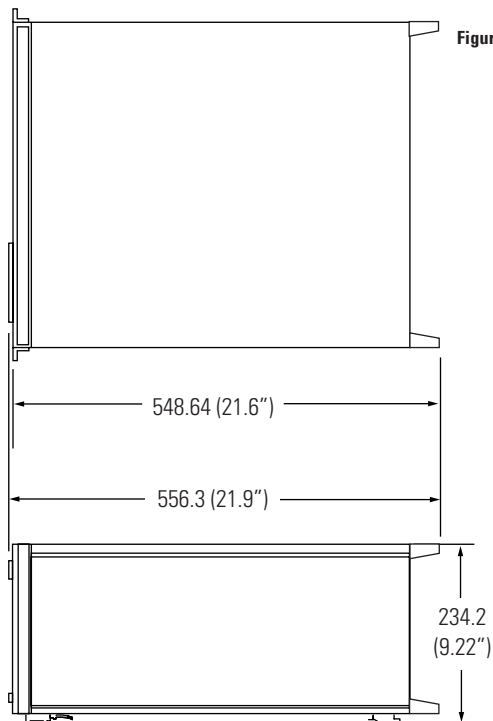
Figure 6.6. Exterior dimensions for the 16700A Series mainframe.
