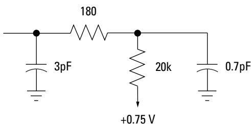
Figure 6.16. E5380A input equivalent probe load.
