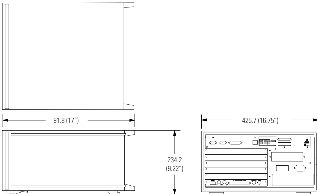
Figure 6.3. Exterior dimensions for the 16700B Series mainframe.
