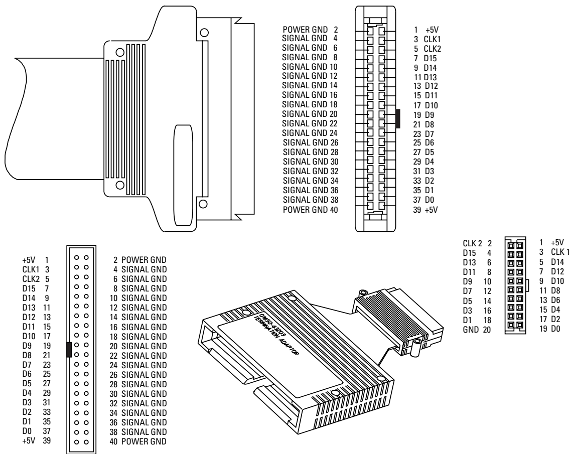
Figure 6.7. Pinout for state/timing module pod cable and 100 KΩ termination adapter. (Agilent 01650-63203)
