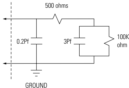
Figure 6.13. Equivalent probe load for the Agilent 16517A/18A.
