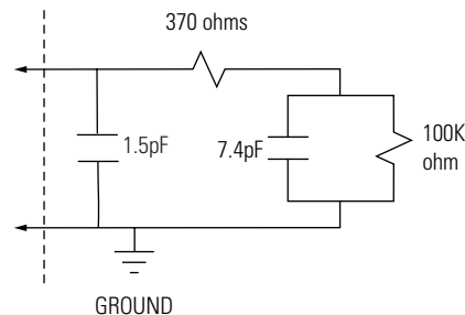
Figure 6.12. Equivalent probe load for the Agilent 16557D, 16710A, 16711A and 16712A, general-purpose lead set.
