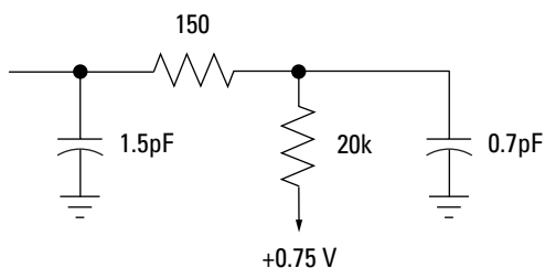
Figure 6.15. E5378A, E5379A input equivalent probe load.
