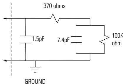
Figure 6.14. Equivalent probe load for the Agilent 16715A, 16716A, 16717A, 16718A, 16719A, 16750A, 16751A, 16752A general-purpose lead set.
